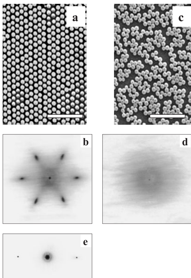
Figure 2. a) Scanning electron micrograph and b) laser diffraction photograph produced by the 2D colloid crystal grown by electrodeposition on a patterned substrate. A collimated laser beam ( \lambda=442 nm) illuminated the crystal at normal incidence and a diffraction pattern was observed on a screen placed behind the sample. For clarity, the negative of the laser diffraction image is shown. c) Scanning electron micrograph and d) laser diffraction image obtained from a colloid crystal grown onto a nonpatterned ITO substrate. e) Laser diffraction pattern produced by the pattern alone. The scale bar is 5 \mu m.
