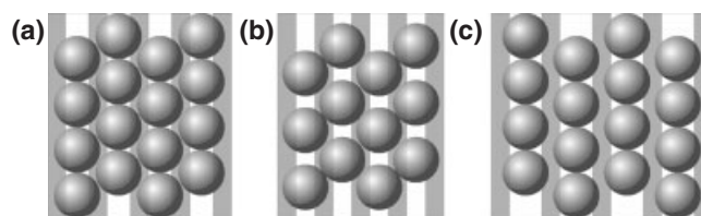
Figure 1. a) Close-packed 2D colloid crystal on a patterned surface with perfectly matched pitch A = (\sqrt{3}/2)D . Because the pitch of the pattern is smaller than microsphere diameter, the relative position of beads in adjacent rows is offset by half of a particle diameter. b) Colloid crystal grown onto a pattern surface with A < (\sqrt{3}/2)D . c) Colloid crystal grown onto a patterned surface with A > (\sqrt{3}/2)D .
