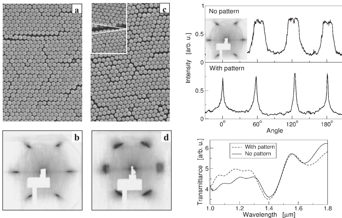
Figure 4. a) SEM and b) laser diffraction photograph (negative) of colloid crystals grown by the meniscus method [2c] on a silicon patterned substrate with ribs parallel to the direction of growth. The diffraction pattern was observed in reflection, since the silicon substrate did not permit transmission of light; the sample and its holder can be seen in front of the diffraction pattern. c) SEM image and d) laser diffraction photograph of a colloid crystal grown under identical conditions on a non-patterned substrate. The inset shows a grain boundary in the same sample: the orientation of the lattice in the two grains differ by an angle of 17^\circ . The scale bar is 5 \mu\text{m} . e) Intensity versus angle in the laser diffraction photos (b,d); the light intensity is measured along the circle arc shown in the inset. f) Transmittance of both samples (plotted on the same scale), measured at normal incidence with an infrared spectrophotometer.
